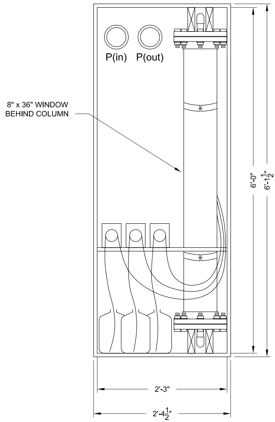
FRONT VIEW
