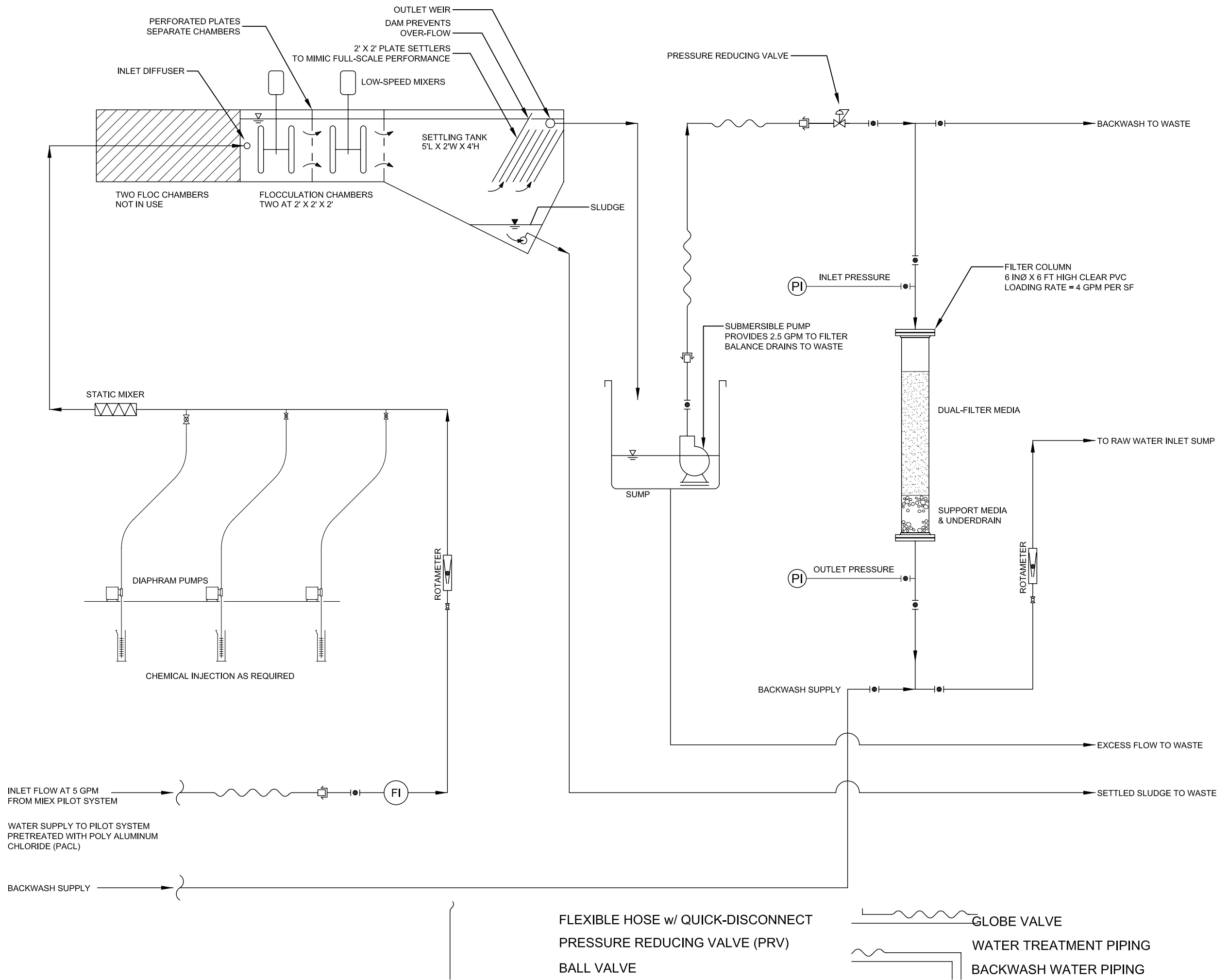
PROPOSED PILOT TEST FLOW DIAGRAM
