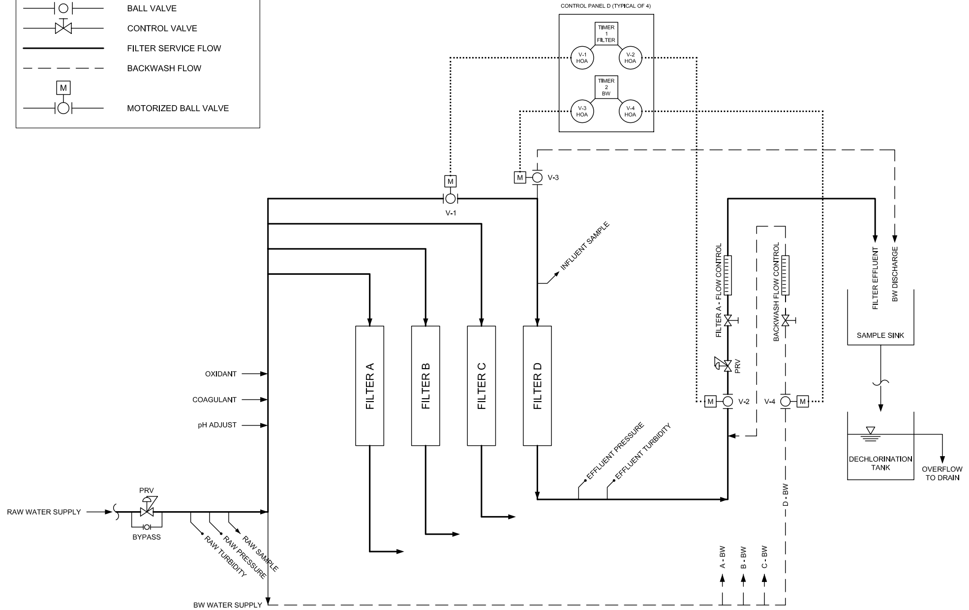
PILOT SYSTEM FLOW DIAGRAM BLUELEAF, INCORPORATED 508.248.7094
